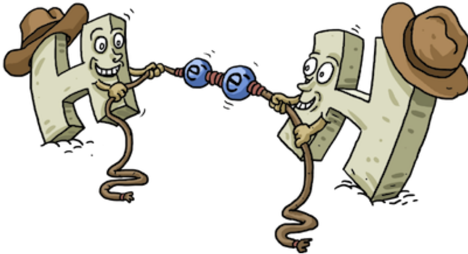
Non-Polar Covalent Bond
